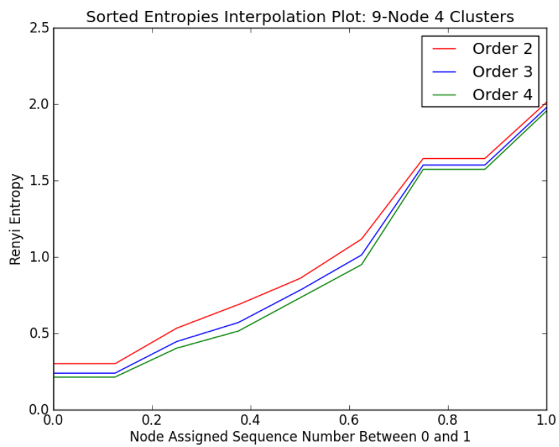
Figure 3.5 Entropy Spectra of 9-Node Network shown in Figure 3.4 These are the interpolation functions between 0 and 1 for Renyi entropies of order 2, 3, and 4 ( I_2 , I_3 , I_4 )
